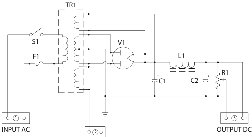
POWER SUPPLY
